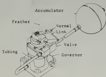
FIGURE 7-15. Unfeathering system.
